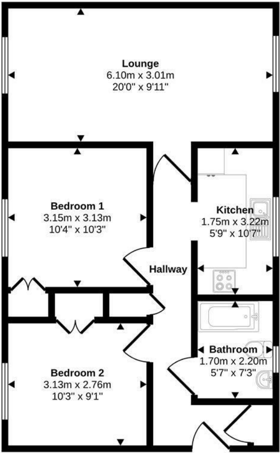
Floorplan
