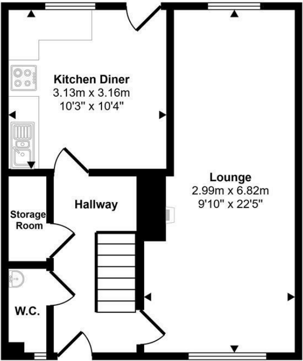
Ground Floor Approx 39 sq m / 421 sq ft
