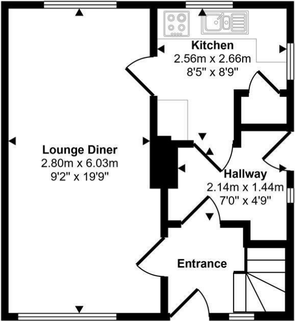
Ground Floor Approx 33 sq m / 361 sq ft
