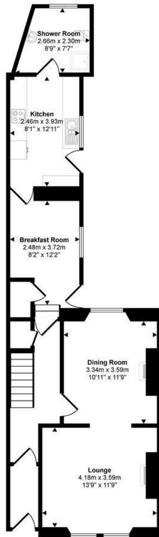
Ground Floor Approx 68 sq m / 729 sq ft
